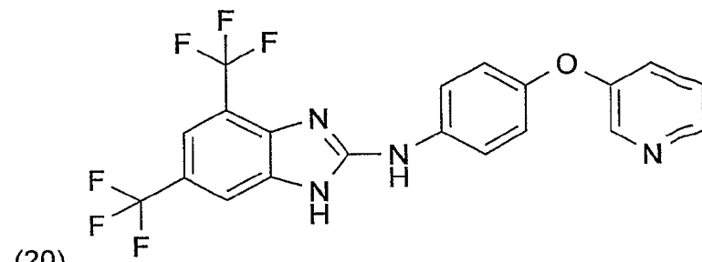
(20) (4,6-Bis-trifluoromethyl-1H-benzimidazol-2-yl)-[4-(pyridin-3-yloxy)-phenyl]-amin
